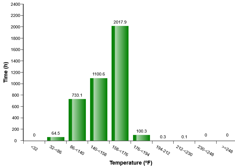
Transmission oil, temperature distribution (h)
